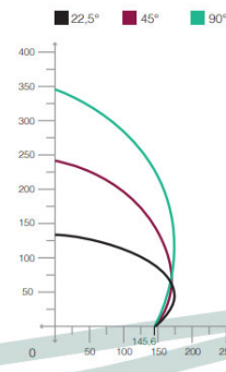
Cutting capacity with tilting of heads compared to the horizontal axis
